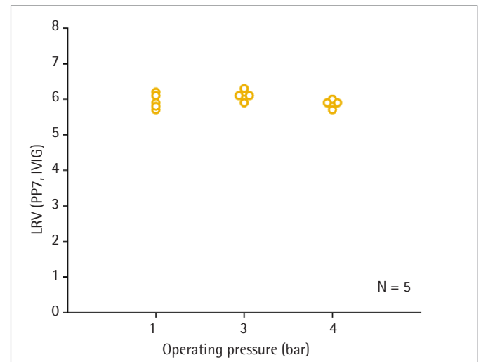
Figure 30: Different operating pressures on PP7 retention at 75% blocking tested for Virosart® HF
