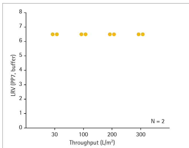
Figure 32: The impact of pressure pulsation tested on PP7 retention
