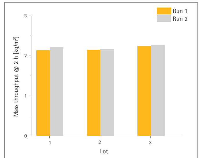
Figure 5: Product throughput for 3 different lots of Virosart® HF filter tested in duplicate runs
