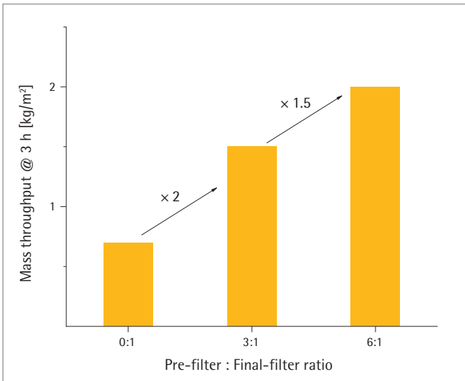
Figure 16: Optimization of adsorptive pre-filter area can improve overall virus-filter throughput
