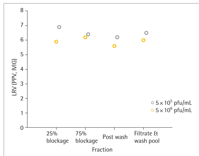
Figure 21: Retention of PPV at 25% and 70% blockage as well as post wash
