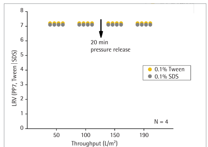
Figure 35: Impact of surface active ingredients such as SDS and Tween on PP7 retention of Virosart® HF
