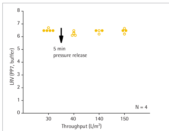
Figure 31: Impact of pressure release on PP7 retention of Virocart® HF
