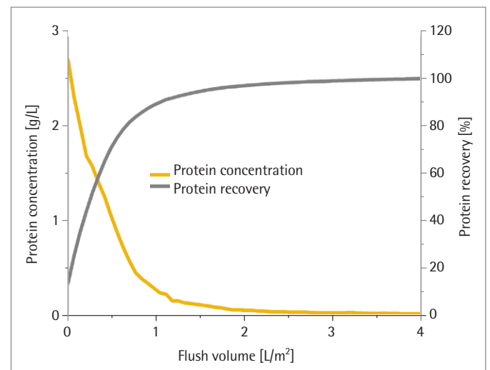
Figure 11: Post-flushing volume for Virosart® HF
