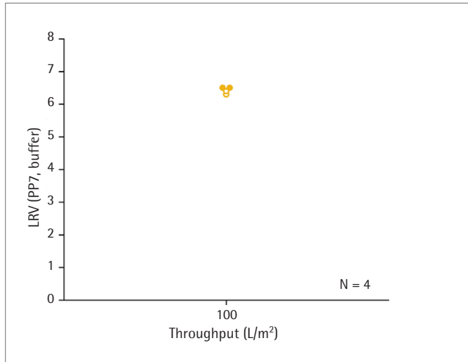
Figure 40: No effect of mechanical stress transport condition on PP7 retention
