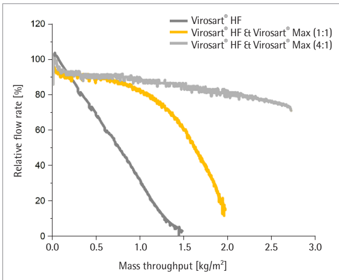
Figure 15: Virus filter throughput can be increased by increasing the adsorptive pre-filtration area
