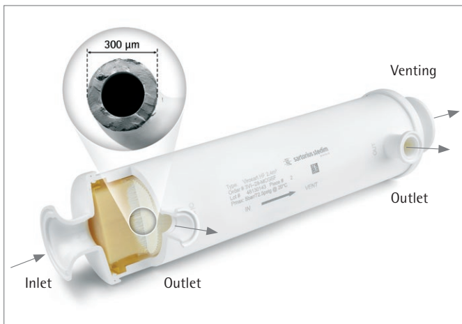
Figure 1: Virosart® HF device set-up
