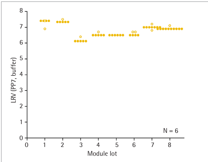
Figure 24: Robust and consistent PP7 retention for Virosart® HF lab modules (5.0 cm 2 ) confirmed for 8 module lots with 6 filters each tested in buffer
