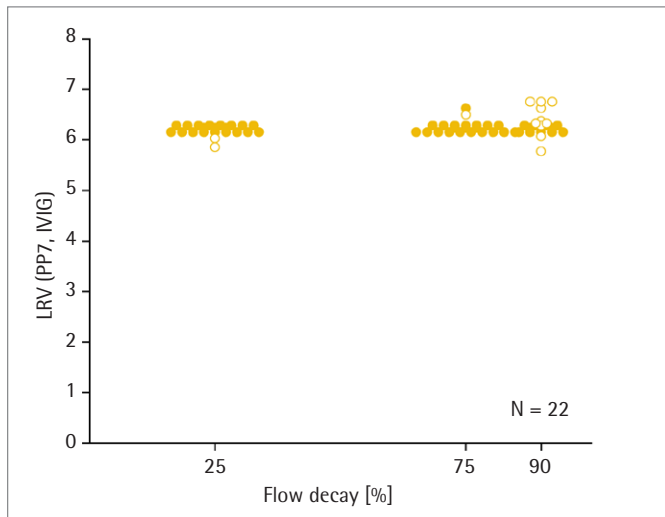
Figure 28: PP7 retention tested at different levels of flow decay for Virosart® HF
