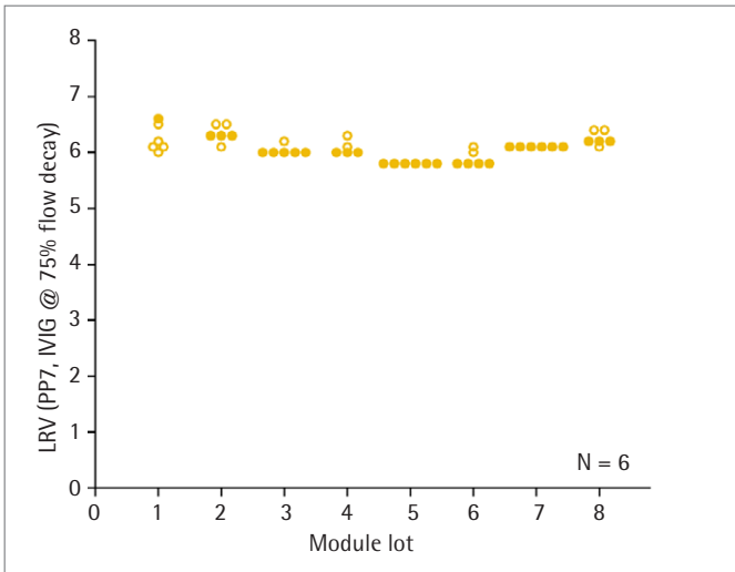
Figure 25: Robust and consistent PP7 retention for Virosart® HF lab modules (5.0 cm 2 ) confirmed for 8 module lots with 6 filters each tested at 75% blocking using IVIG.
