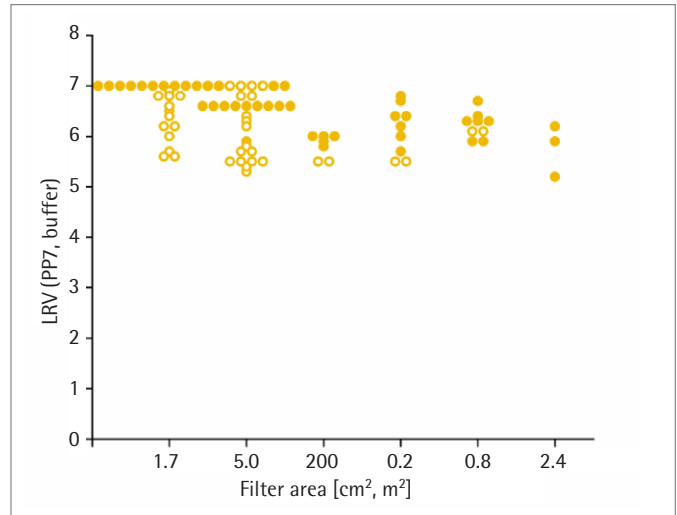
Figure 26: PP7 retention for the whole module family of Virosart® HF in buffer
