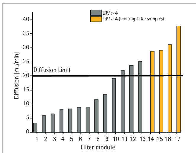
Figure 44: Correlation of PP7 retention and diffusion value for Virosart® HF process modules (0.8 m 2 )
