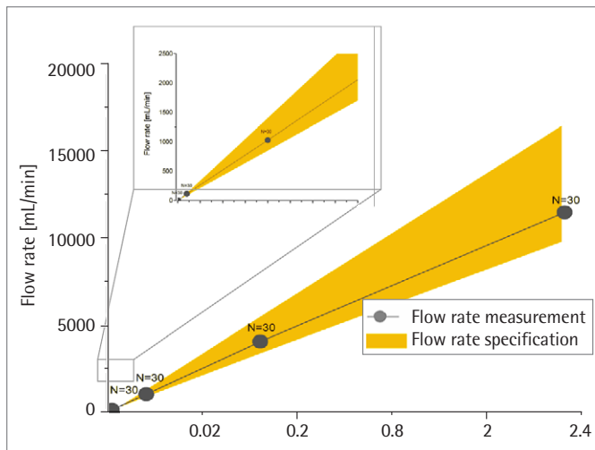
Figure 9: Average of water flow rates at 2.0 bar | 30 psi through the entire product family of Virosart® HF
