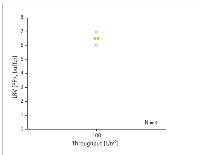
Figure 38: Effect of thermal stress transport condition on PP7 retention investigated
