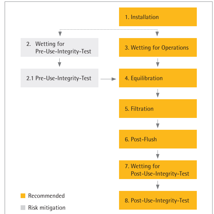
Figure 2: Process steps during virus filtration
