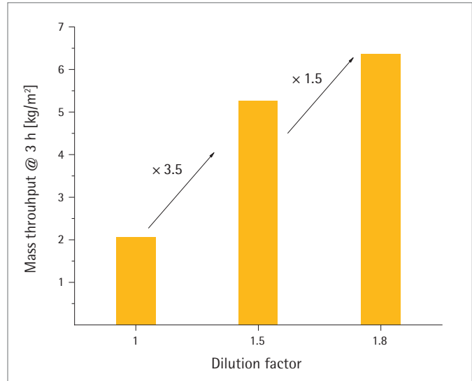
Figure 17: Dilution of feed stream impacting product throughput over the virus filter
