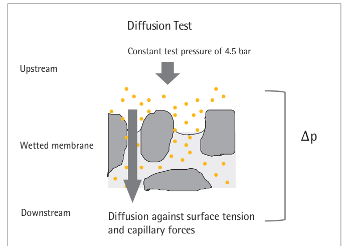
Figure 41: Schematic drawing of the Integrity Test based on diffusion. Applying test pressure to upstream side results in gradient from upstream side to downstream side, thus a net flux in the direction of filtration. This situation is relevant for integer devices, where the Bubble Point of the membrane has not been reached by the test pressure.
