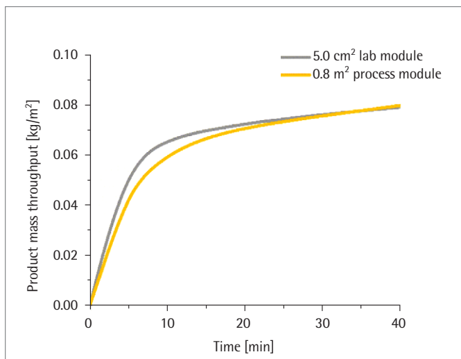
Figure 10: Product mass throughput of the Virosart® HF lab (5.0 cm 2 ) and process module (0.8 m 2 )
