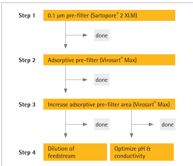
Figure 19: Decision tree for virus filter throughput optimization
