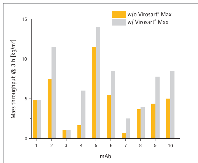
Figure 14: Impact of inline pre-filtration on the overall throughput of Virosart® HF
