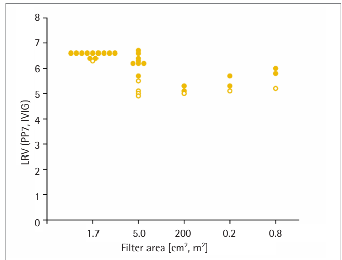
Figure 27: PP7 retention for the whole module family of Virosart® HF in IVIG
