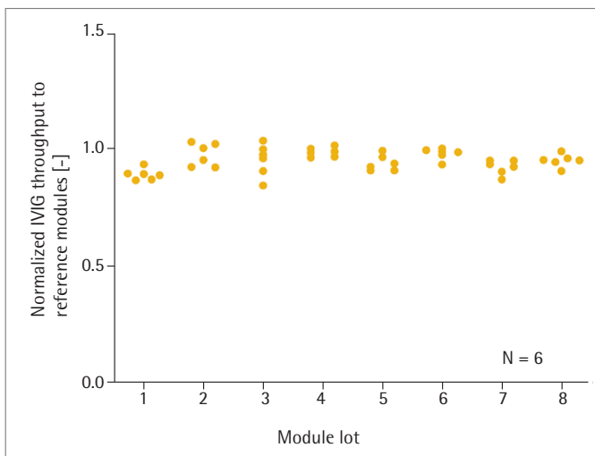
Figure 7: Protein throughput for 42 modules of 8 different module lots of Virosart® HF using IVIG. Protein throughput has been normalized to reference modules
