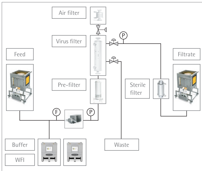
Figure 3: Set-up for a typical virus filtration unit operation
