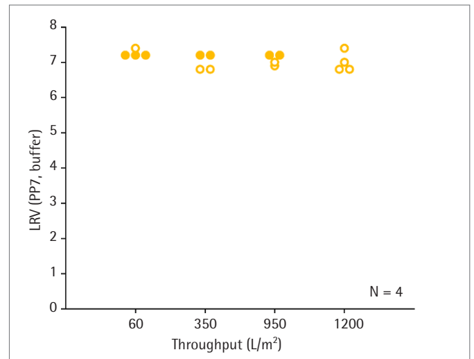
Figure 34: Retention at low pH and high salt concentration during high challenge load
