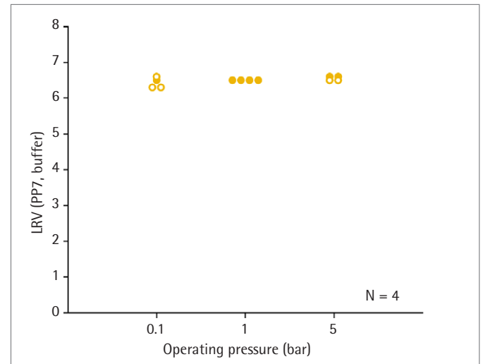
Figure 29: Different operating pressures of 0.1 bar, 1.0 bar and 5.0 bar tested on PP7 retention for Virosart® HF
