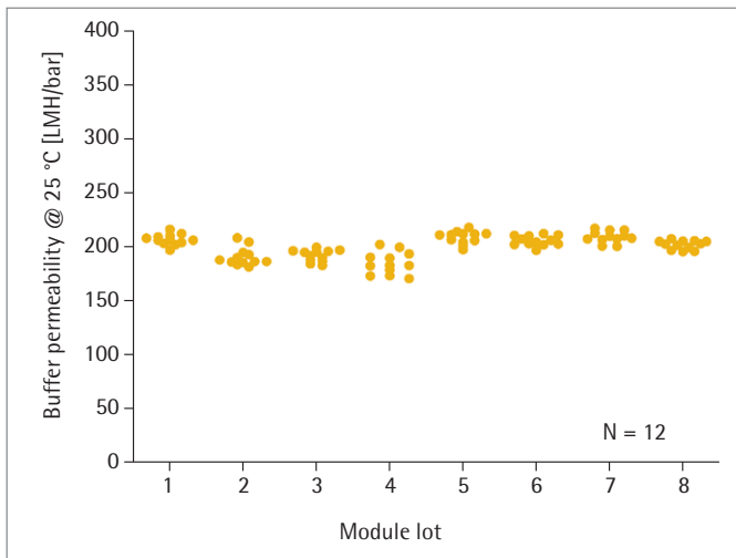
Figure 6: Buffer permeability for Virosart® HF lab modules shown for 96 filters of 8 different lots
