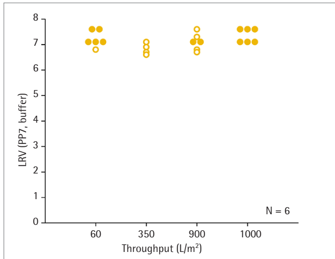
Figure 33: Impact of high load on PP7 retention investigated
