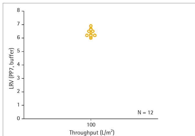
Figure 36: Effect of drop-test on PP7 retention studied with 5.0 cm 2 lab modules
