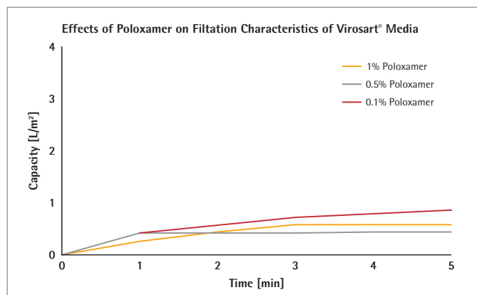
Figure 3: Effect of poloxamers on filtration characteristics through the Virosart ® Media filter in DI water
