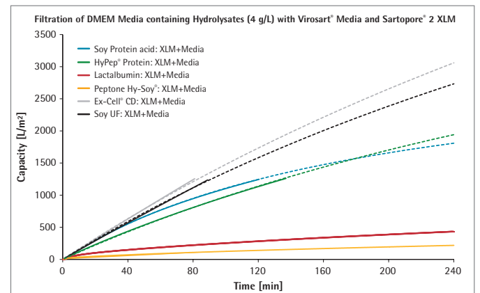
Figure 5: Filtration of six different hydrolysates in DMEM media with Virosart® Media and Sartopore® 2 XLM at constant pressure of 2.0 bar | 30 psi for 240 min filtration.
