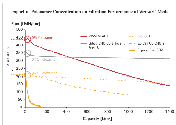
Figure 2: Impact of poloxamer concentration (0–0.2%) with five different media on filtration characteristics of Virosart ® Media at 2.0 bar | 30 psi constant pressure during 4 hour filtration
