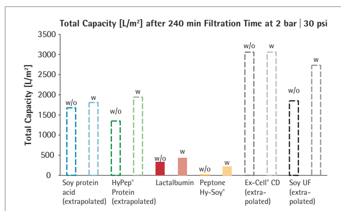
Figure 6: Total capacity after 240 min filtration time at constant pressure of 2.0 bar | 30 psi in duplicate runs w/ and w/o pre-filter
