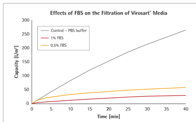
Figure 7: Filtration of FBS through the Virosart® Media filter
