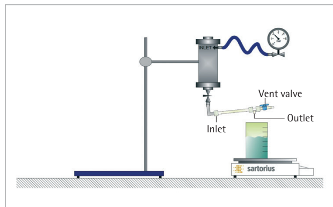
Figure 1: Experimental set-up of small-scale filtration using Virosart® Media lab module 5 cm 2
