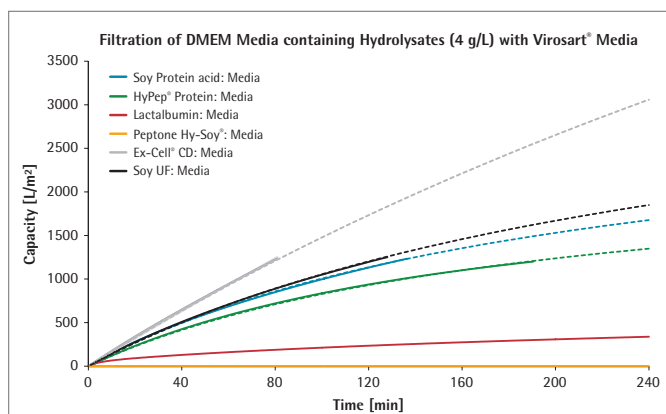
Figure 4: Filtration of six different hydrolysates in DMEM media with Virosart® Media at constant pressure of 2.0 bar | 30 psi for 240 min filtration
